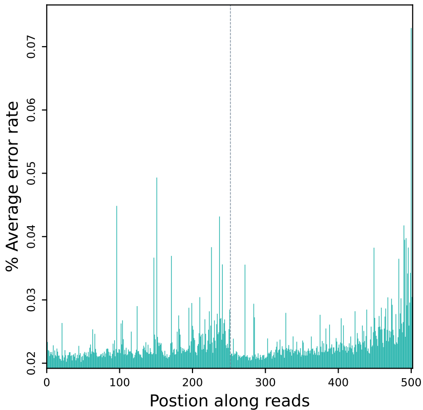
Error rate distribution along reads (R10915)
